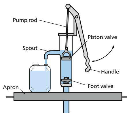
PISTON PUMP
